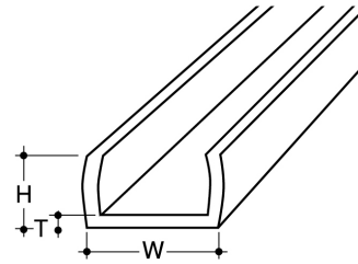
Extruded Unserrated Polyethylene
